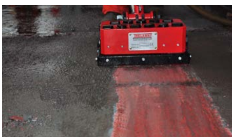
DECK DESCALING
