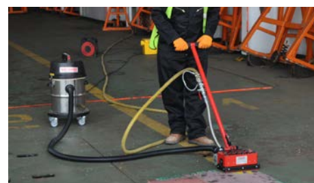
USE WITH KAV30 VACUUM
